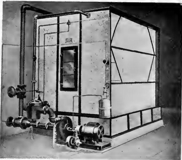
FIG. 7. A TYPICAL AIR WASHER DESIGNED FOR AUTOMATIC HUMIDITY CONTROL
